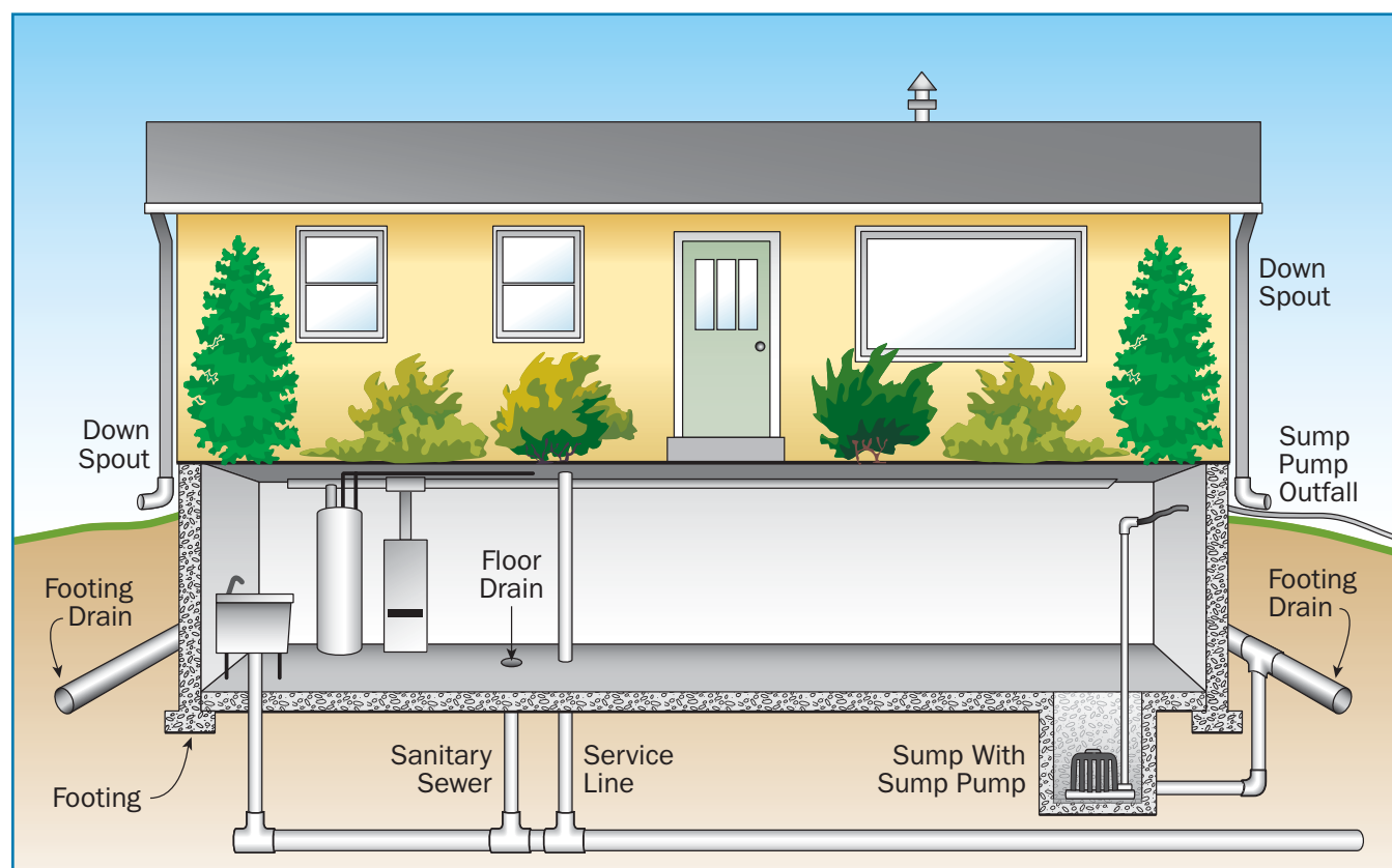
Typical basement drain and sewer arrangement.
